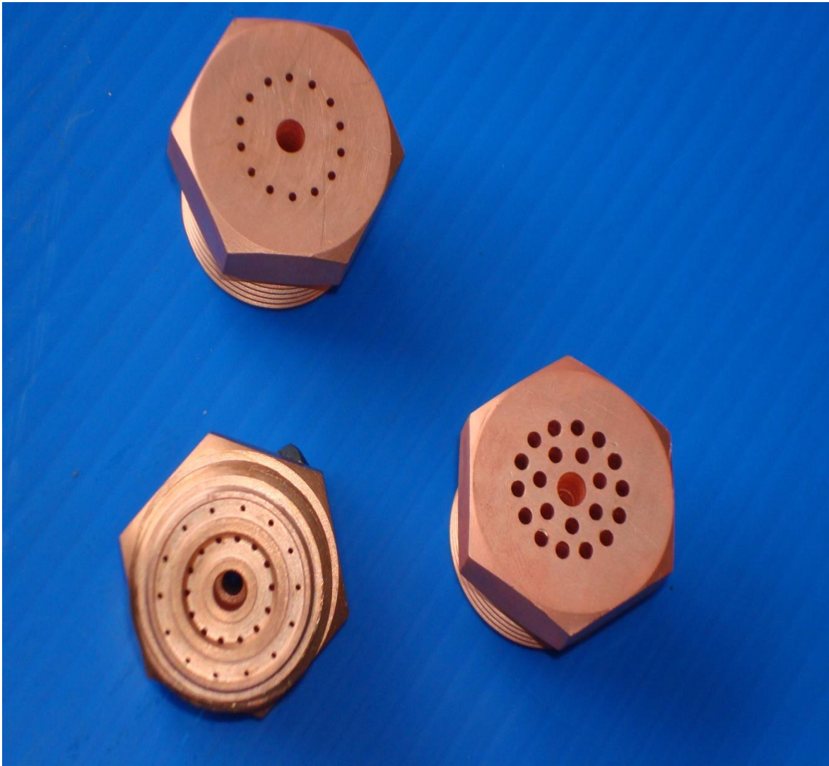
Nozzles
